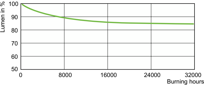
Lumen Maintenance Diagram - MASTER GreenPower Plus 600W EL E40 UNP
